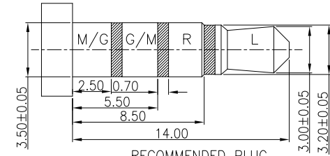
RECOMMENDED PLUG Ø3.5 4 POLE STANDARD PLUG
