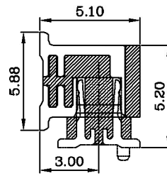
ASSEMBLY
