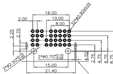
RECOMMENDED PCB LAYOUT (TOP VIEW) GENERAL TOLERANCE:±0.05mm(T=1.60)
