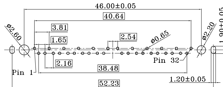
RECOMMENDED PCB LAYOUT(T=3.00±0.10)
