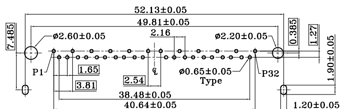
RECOMMENDED PCB LAYOUT(T=2.36±0.08)
