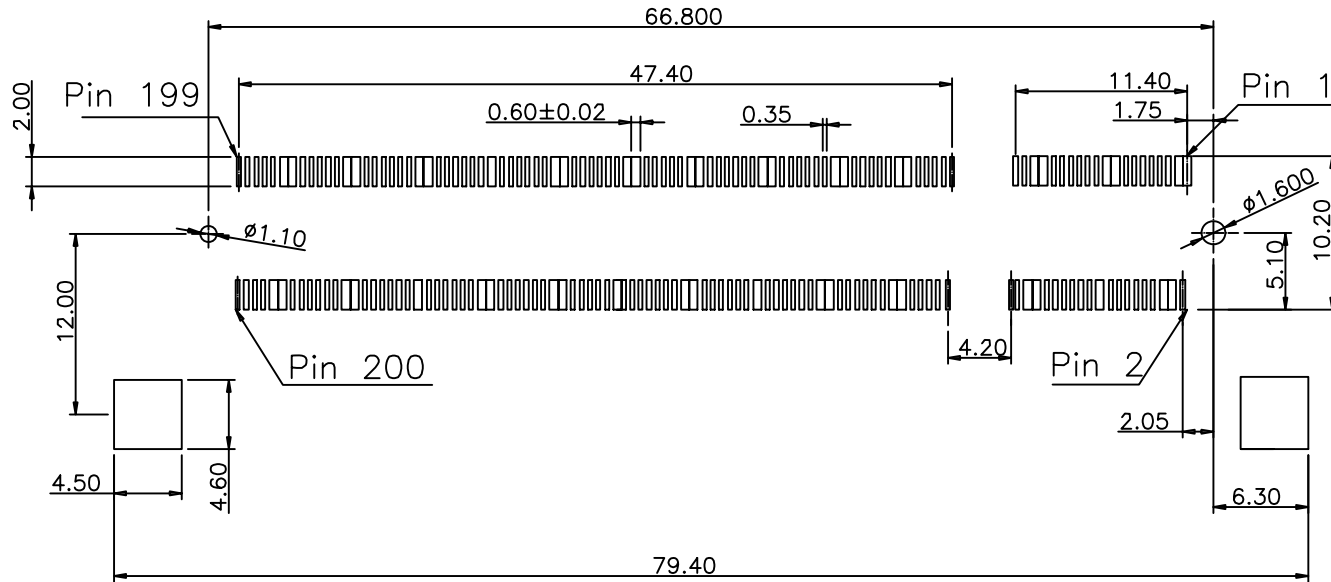
TOP VIEW PCB LAYOUT RECOMMENDED
