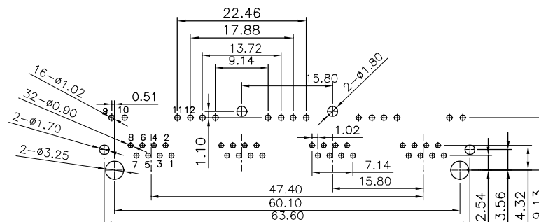
RECOMMENDED P.C.B LAYOUT TOP VIEW (COMPONENT SIDE) TOLERANCE ±0.05
